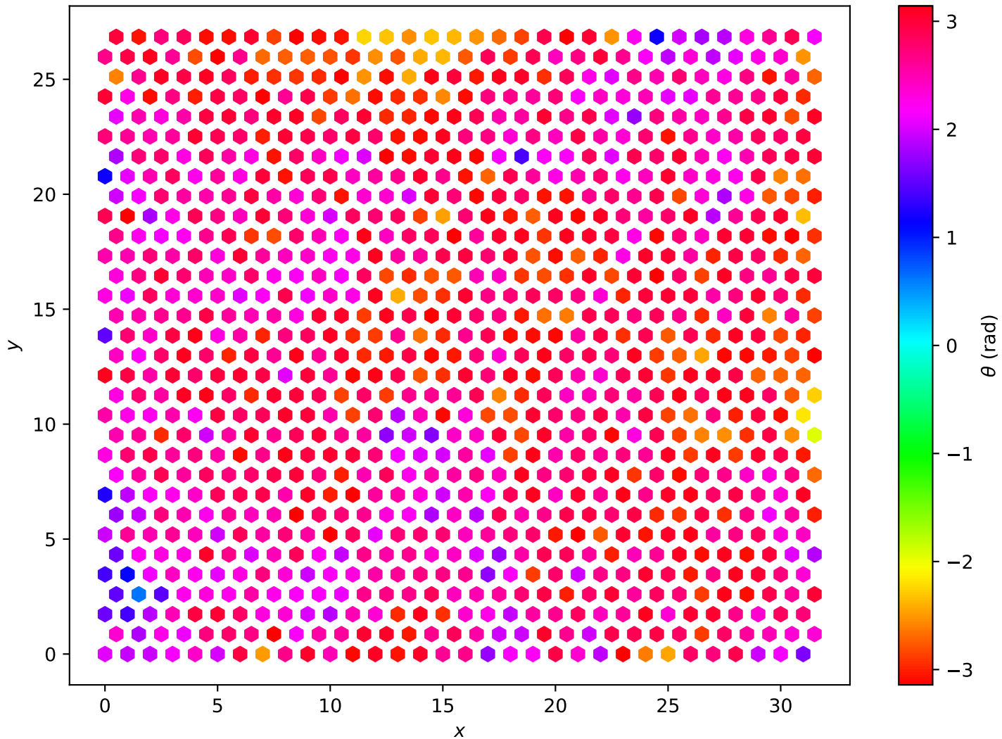
Hexagonal Lattice L=32 , T = 5.00e - 01
