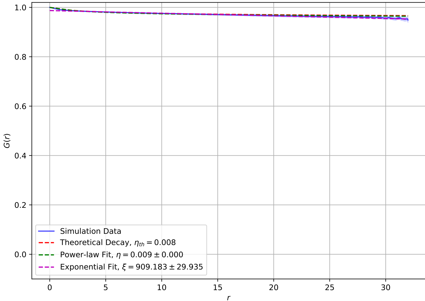
Correlation Function at T = 5.00e - 02 , L = 32
