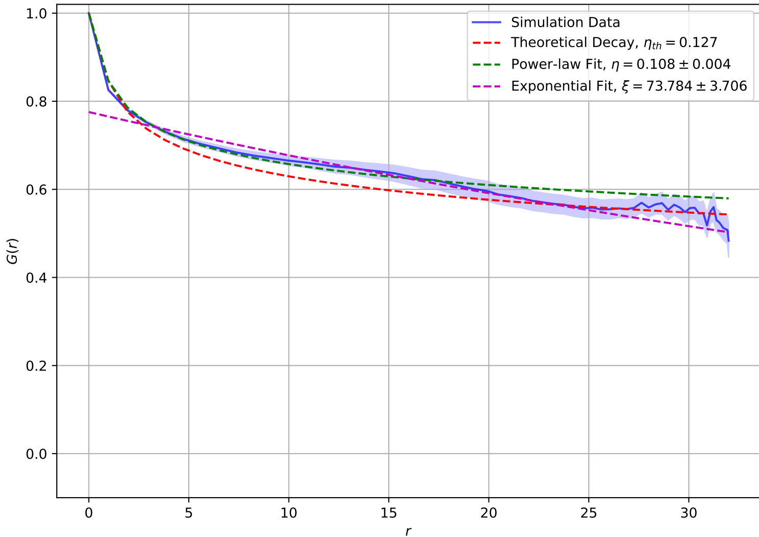
Correlation Function at T = 8.00\text{e} - 01 , L = 32
