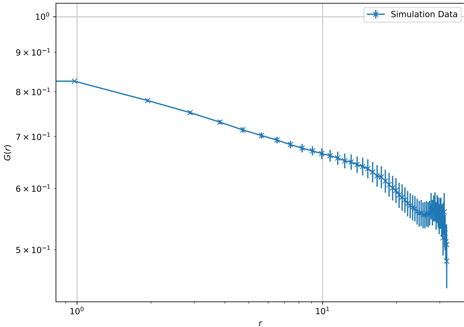
Correlation Function at T = 8.00e - 01 , L = 32 (Log-Log Scale)
