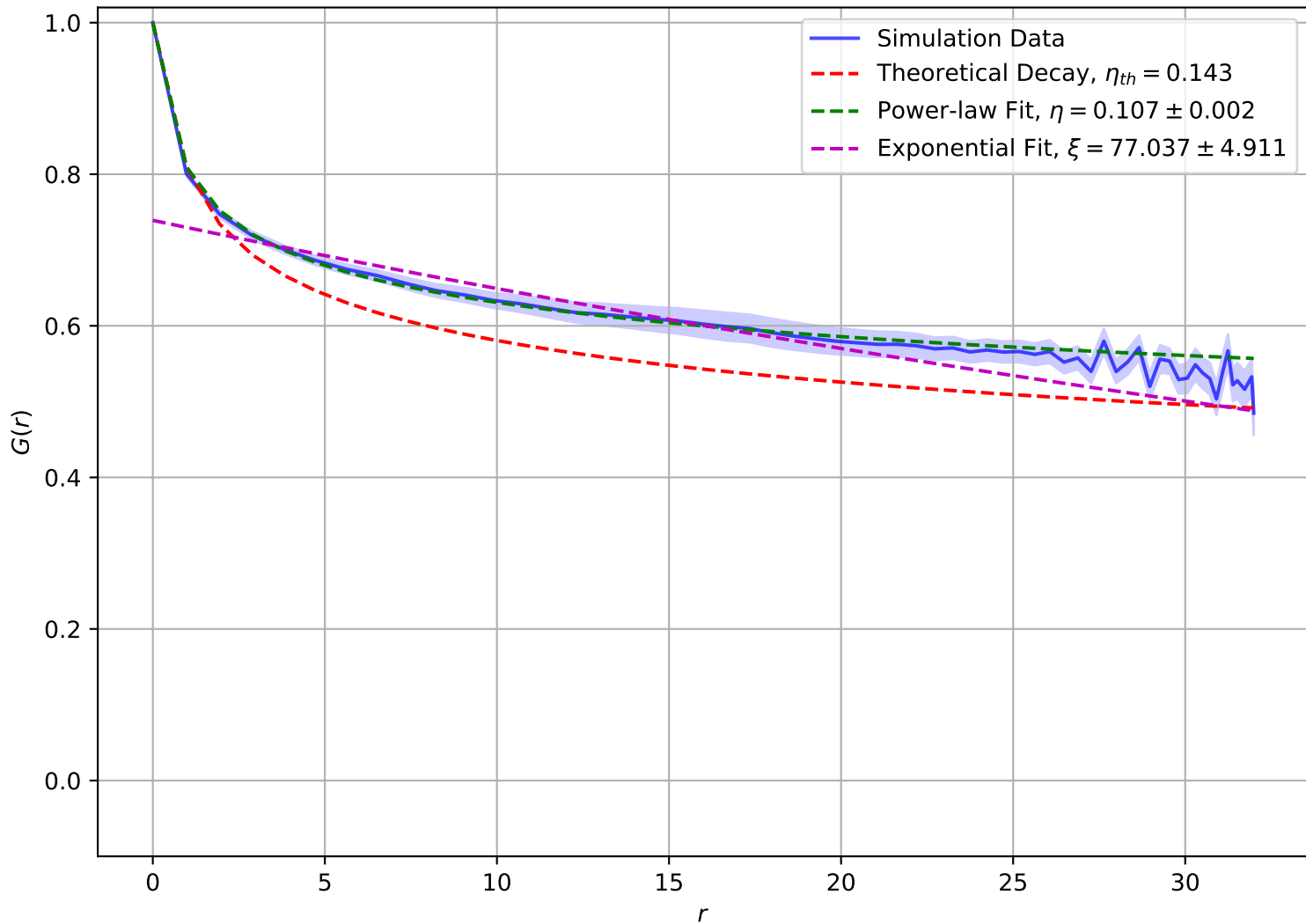
Correlation Function at T = 9.00e - 01 , L = 32
