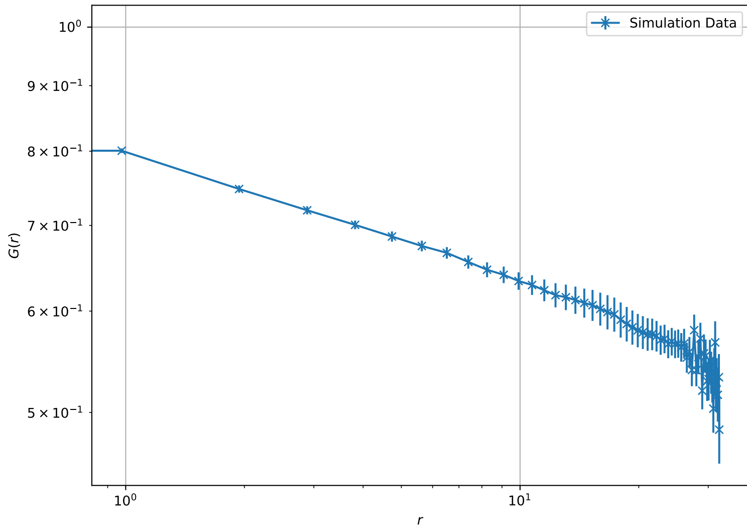
Correlation Function at T = 9.00e - 01 , L = 32 (Log-Log Scale)
