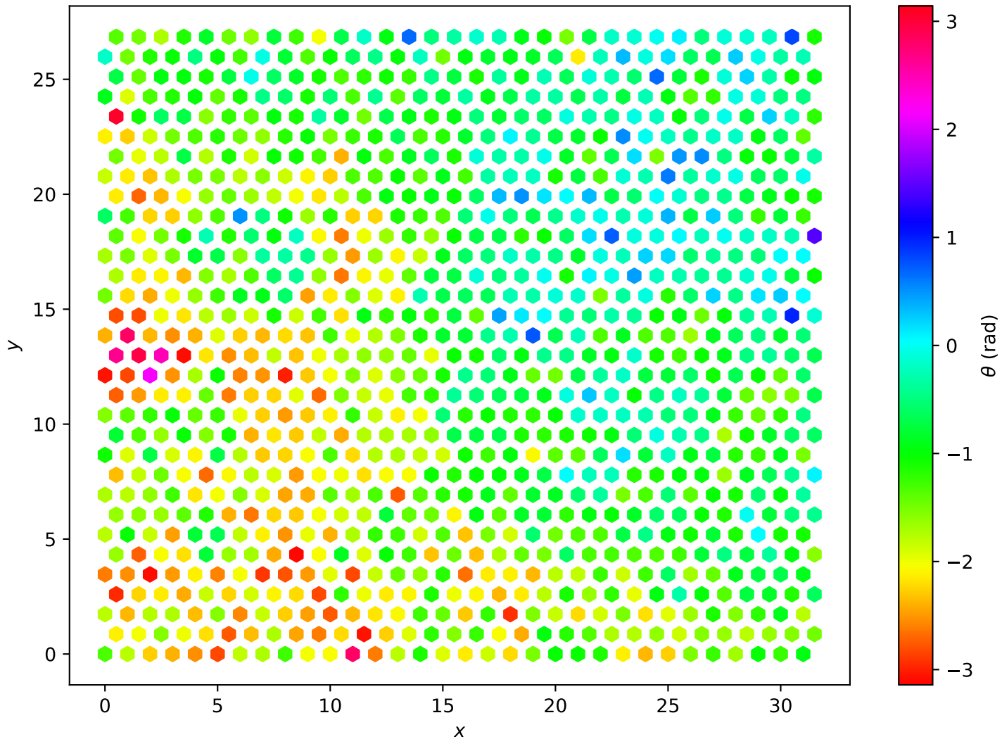
Hexagonal Lattice L=32 , T = 9.00e - 01
