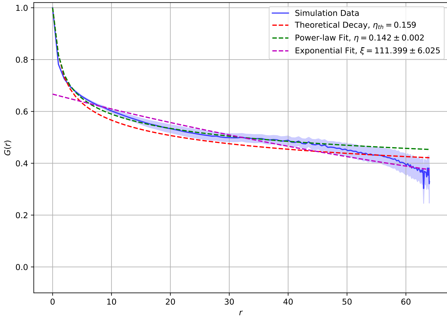
Correlation Function at T = 1.00e + 00 , L = 64
