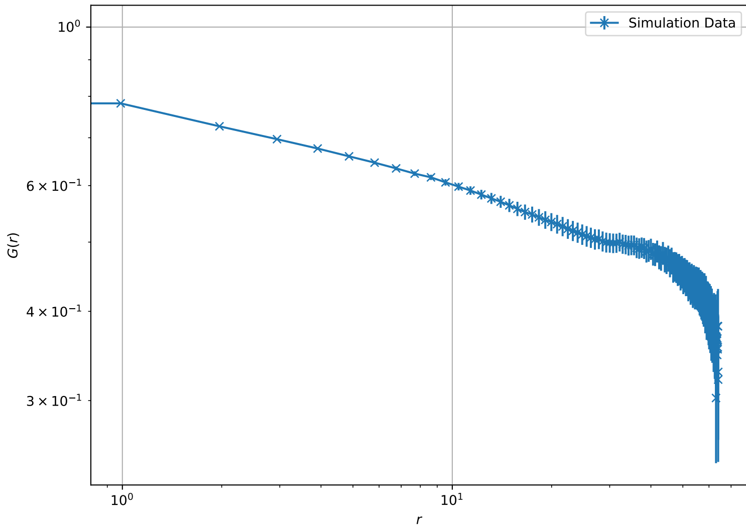
Correlation Function at T = 1.00e + 00 , L = 64 (Log-Log Scale)
