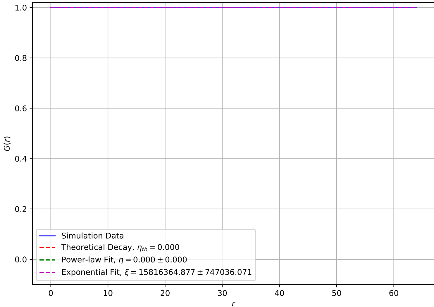
Correlation Function at T = 1.00e - 05 , L = 64
