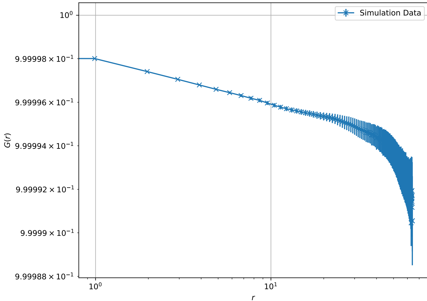
Correlation Function at T = 1.00e - 05 , L = 64 (Log-Log Scale)
