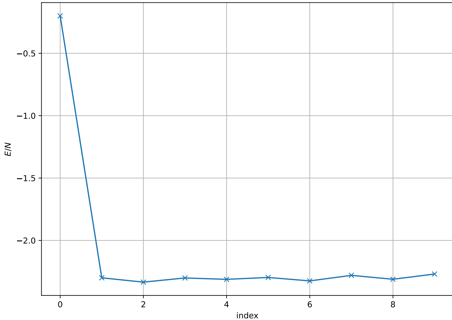
Energy per Site at T = 1.100e + 00 , L = 64
