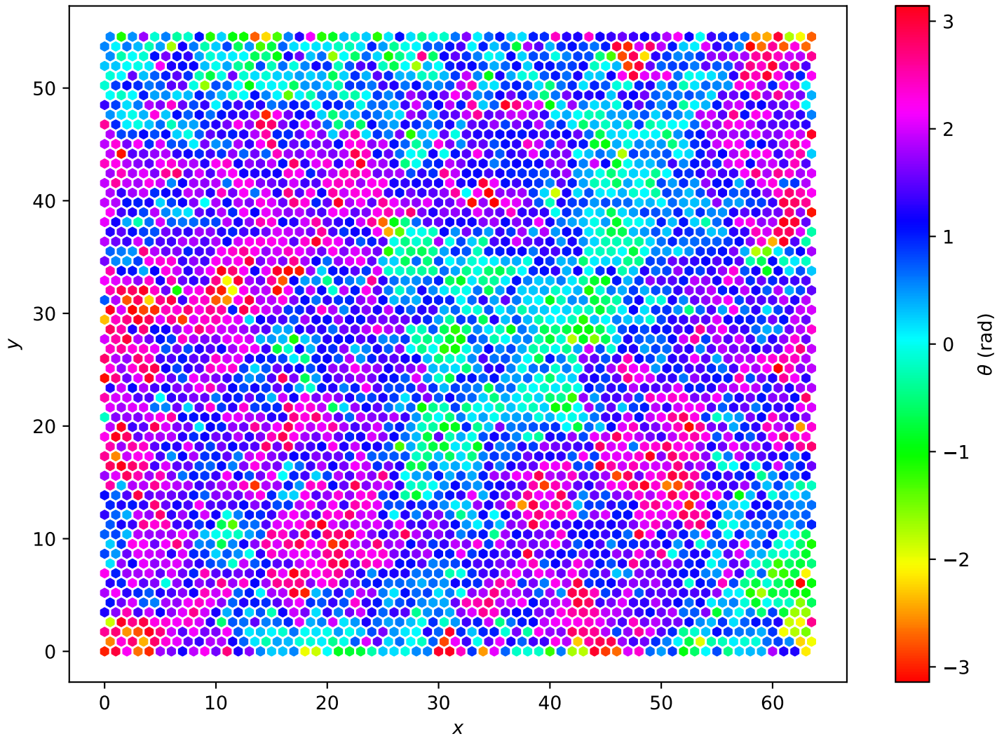
Hexagonal Lattice L=64 , T = 1.30e + 00
