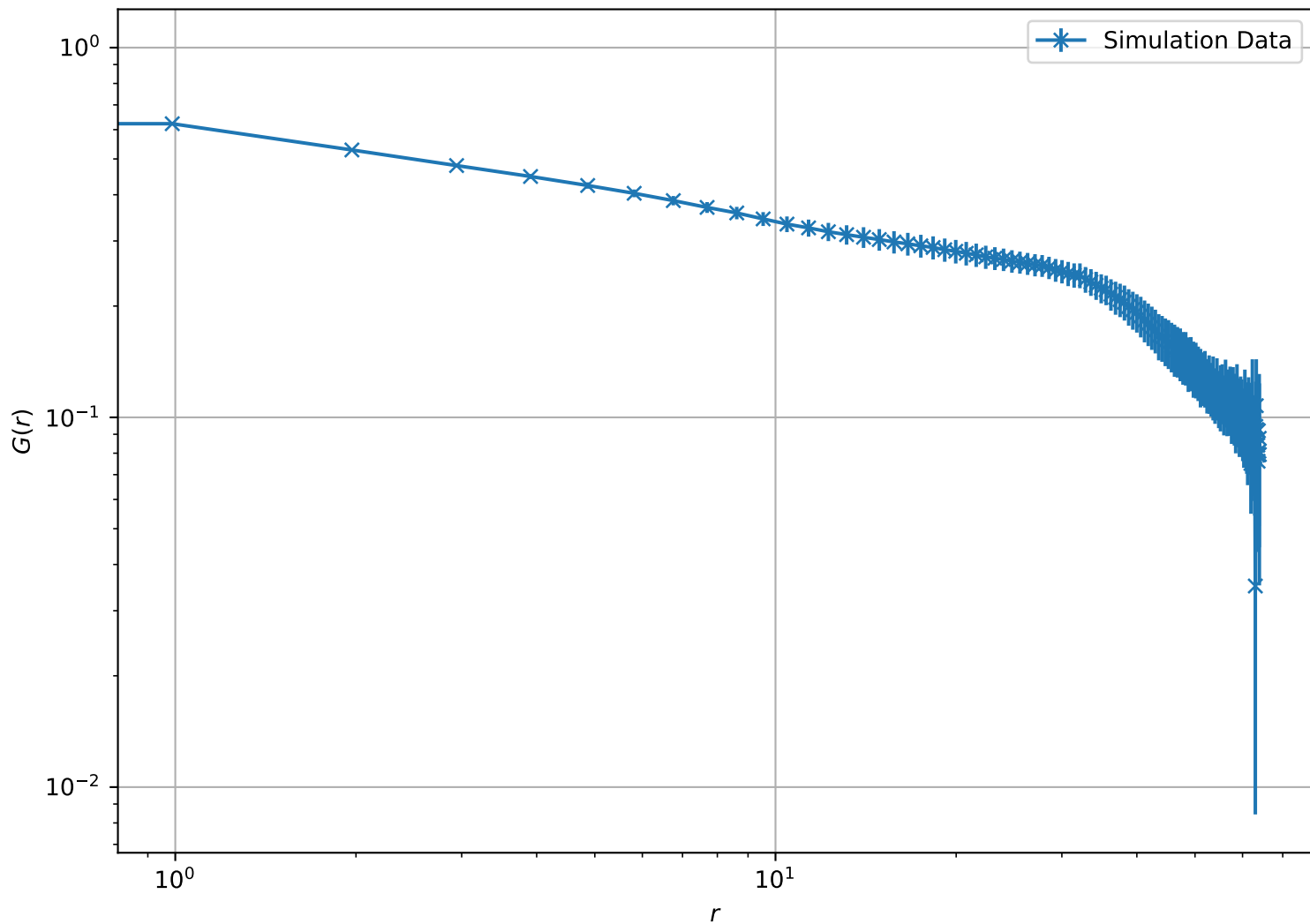
Correlation Function at T = 1.50e + 00 , L = 64 (Log-Log Scale)
