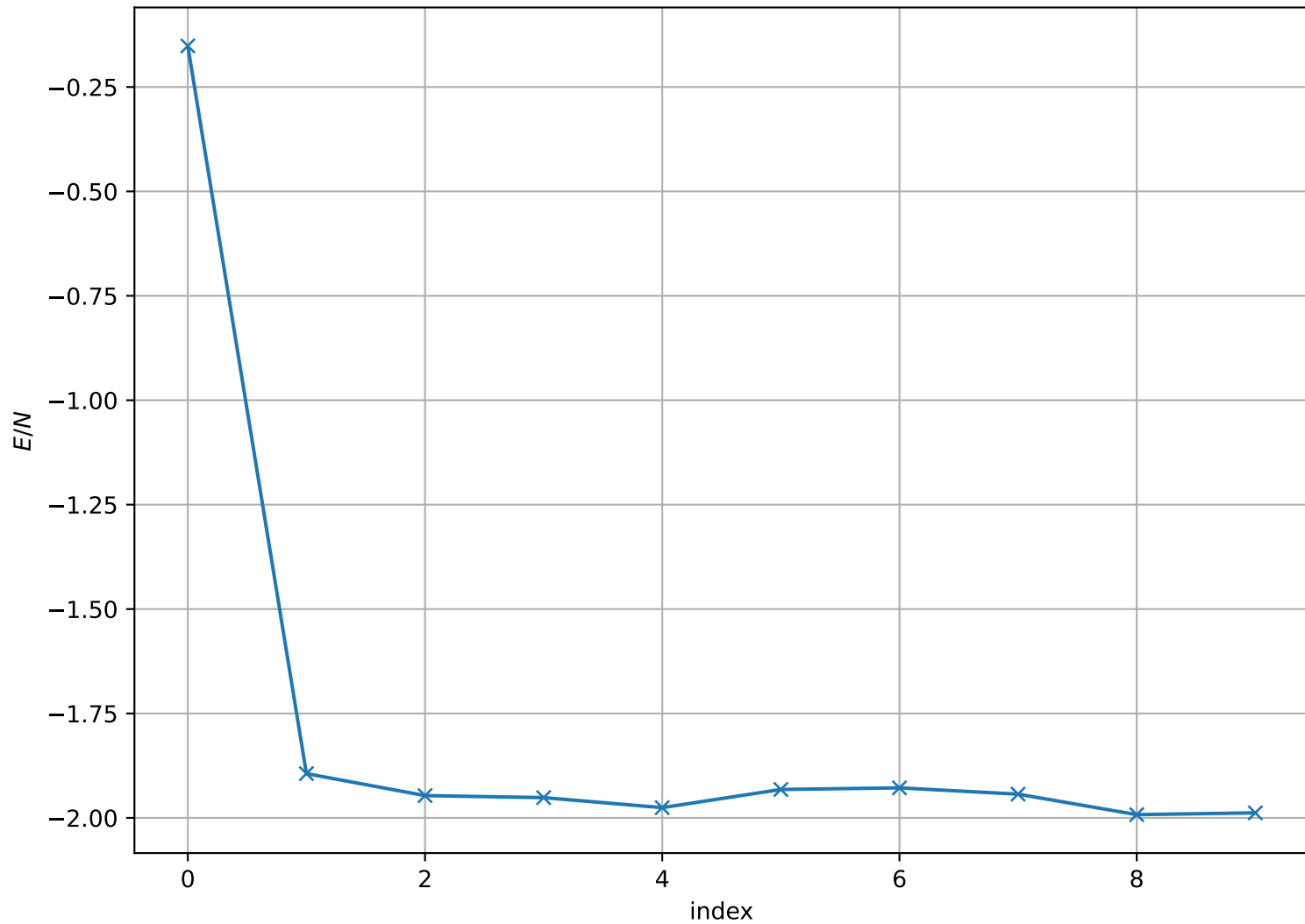
Energy per Site at T = 1.500e + 00 , L = 64
