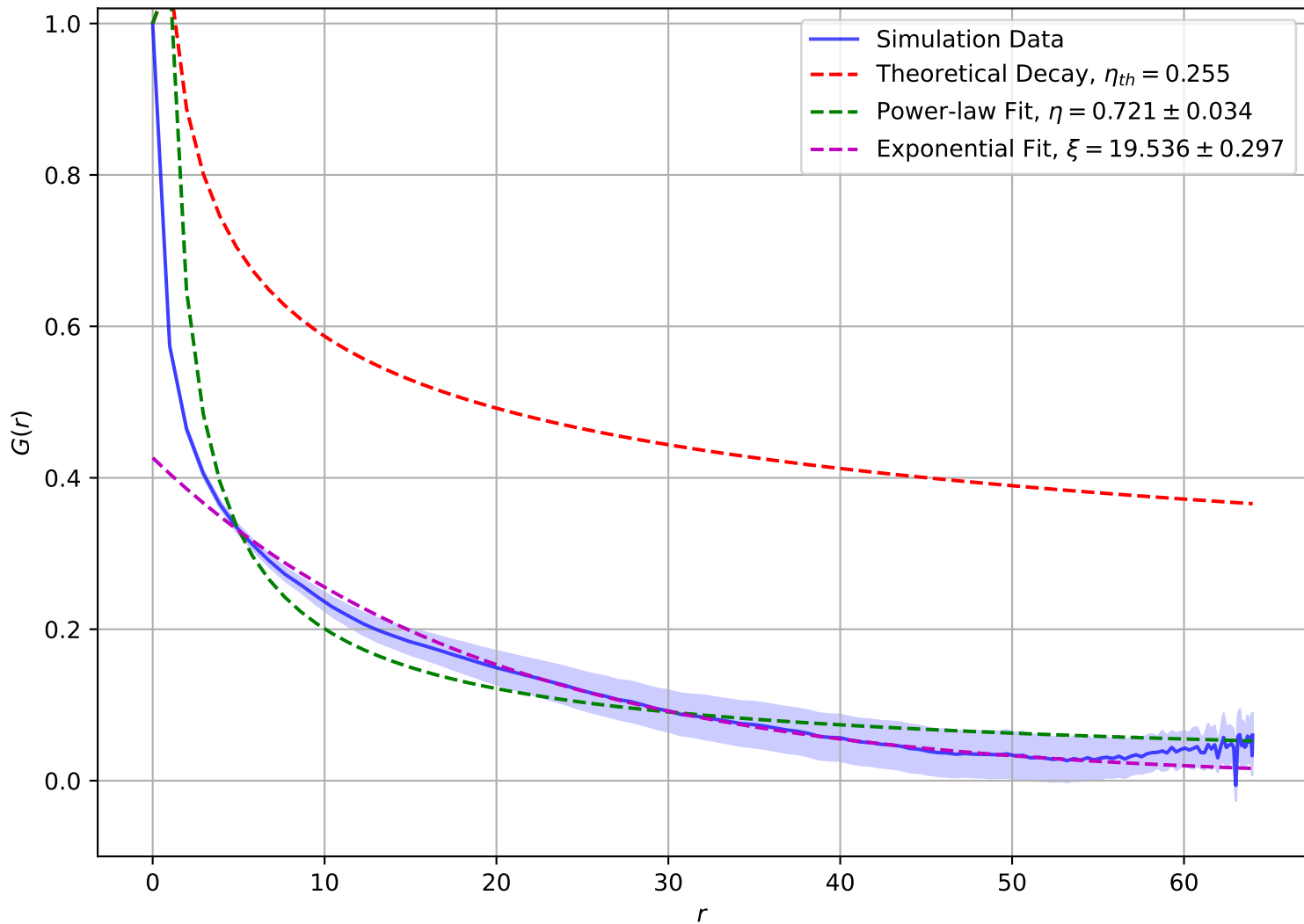
Correlation Function at T = 1.60e + 00 , L = 64
