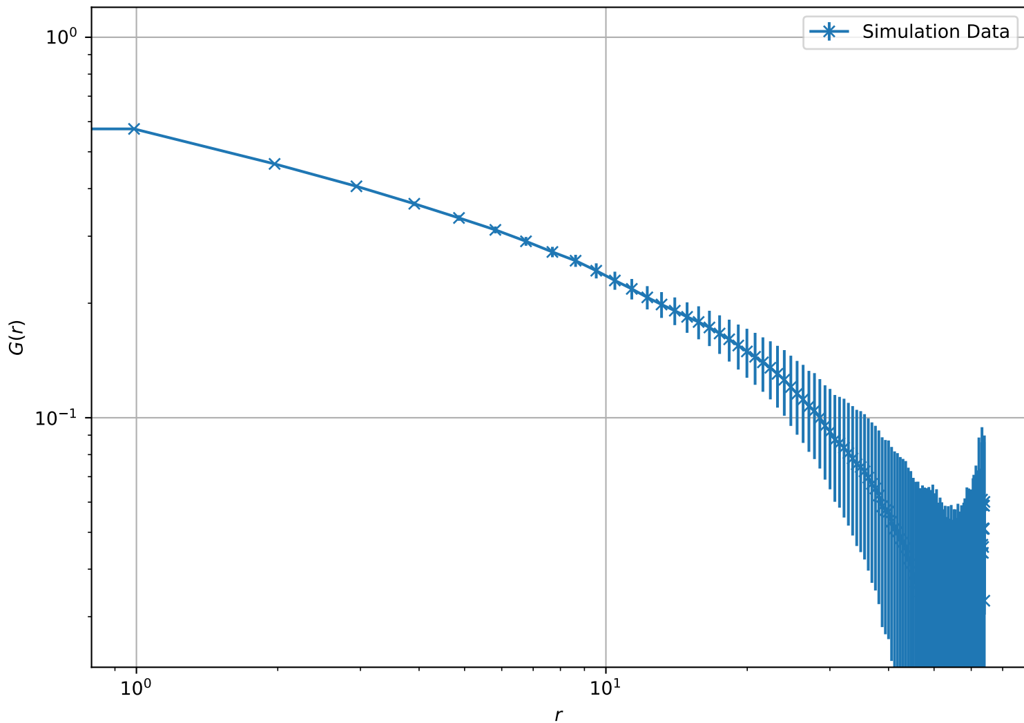
Correlation Function at T = 1.60e + 00 , L = 64 (Log-Log Scale)
