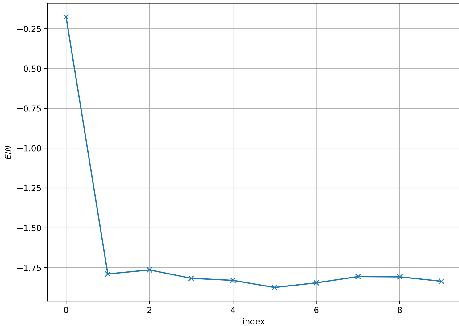
Energy per Site at T = 1.600e + 00 , L = 64
