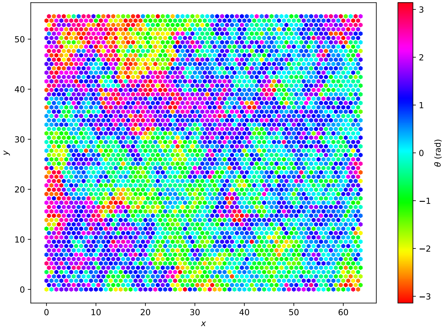
Hexagonal Lattice L=64 , T = 1.60e + 00
