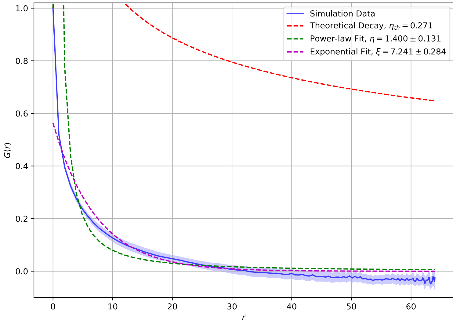
Correlation Function at T = 1.70e + 00 , L = 64
