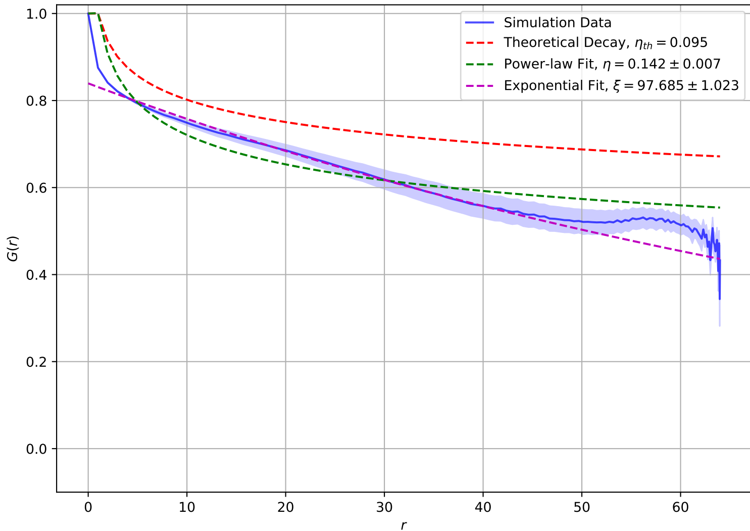
Correlation Function at T = 6.00e - 01 , L = 64
