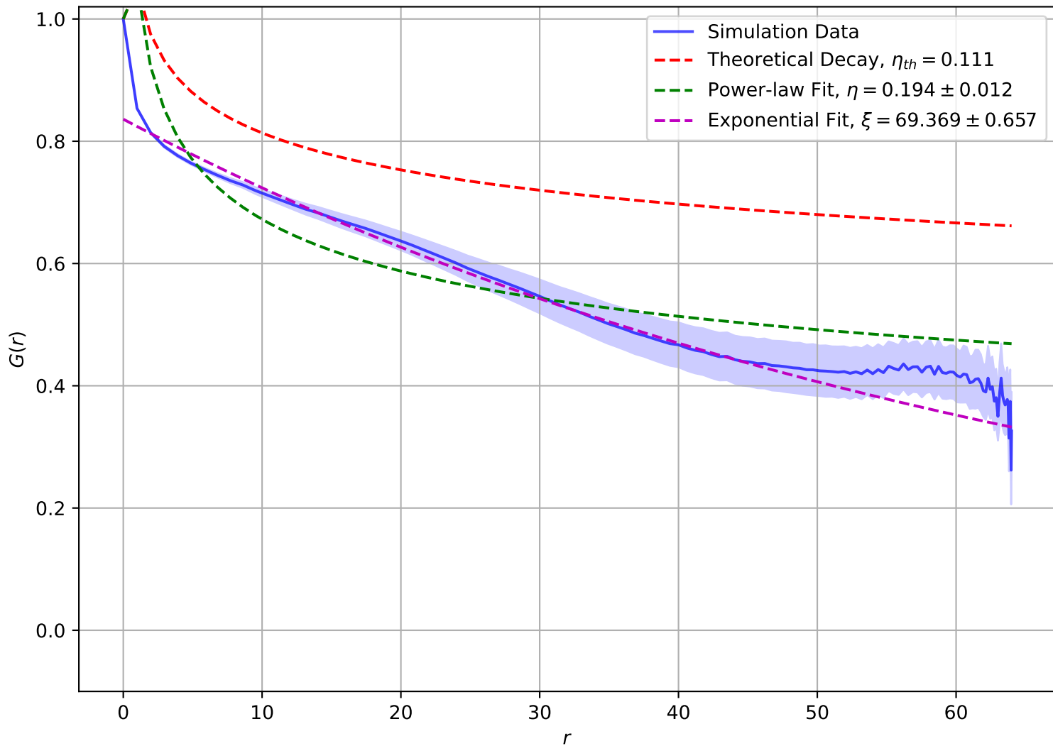
Correlation Function at T = 7.00e - 01 , L = 64
