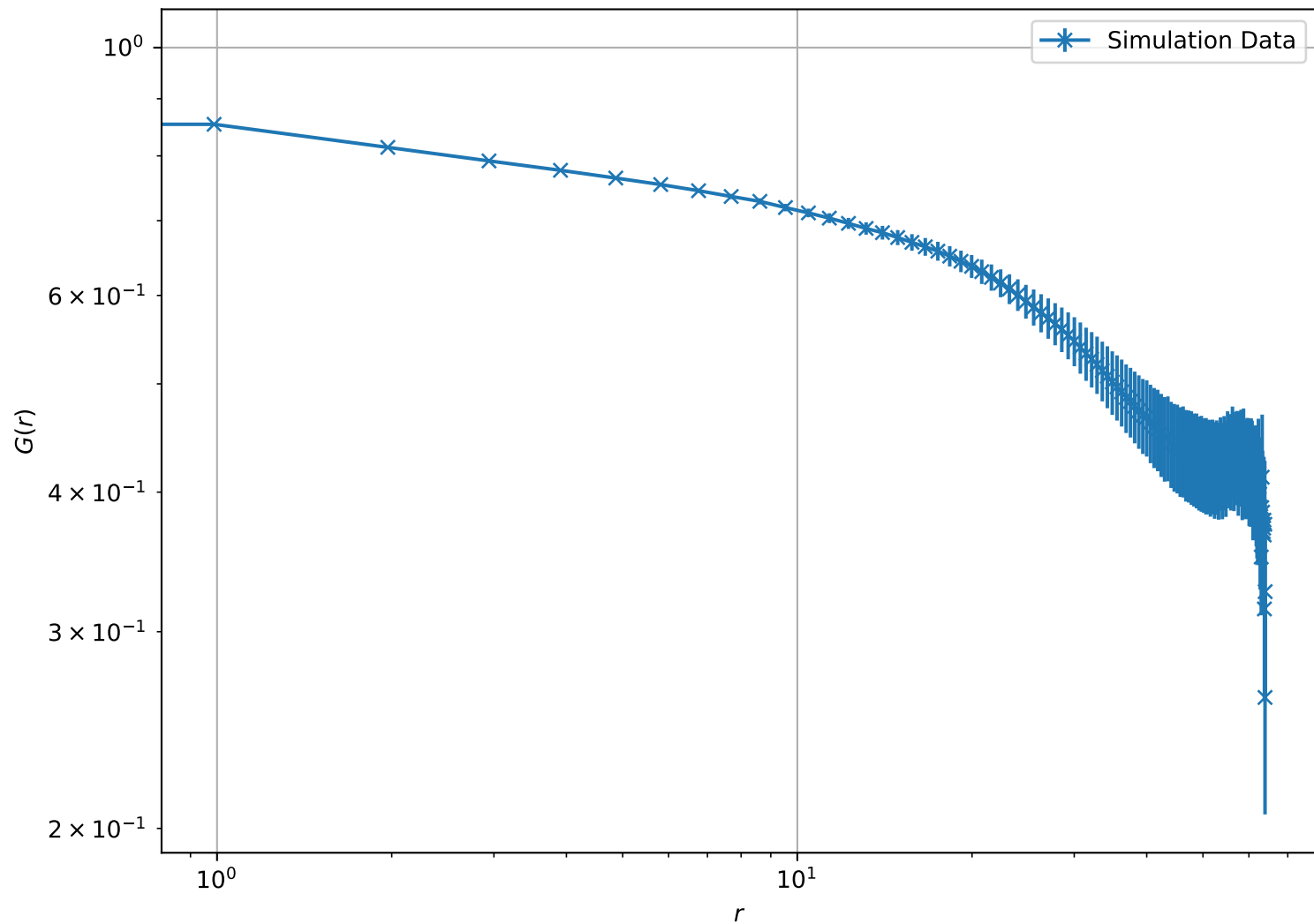
Correlation Function at T = 7.00e - 01 , L = 64 (Log-Log Scale)
