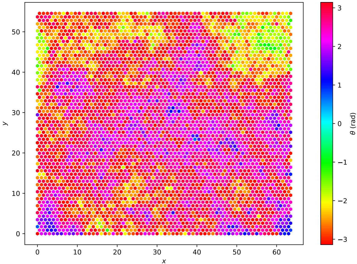
Hexagonal Lattice L=64 , T = 7.00e - 01
