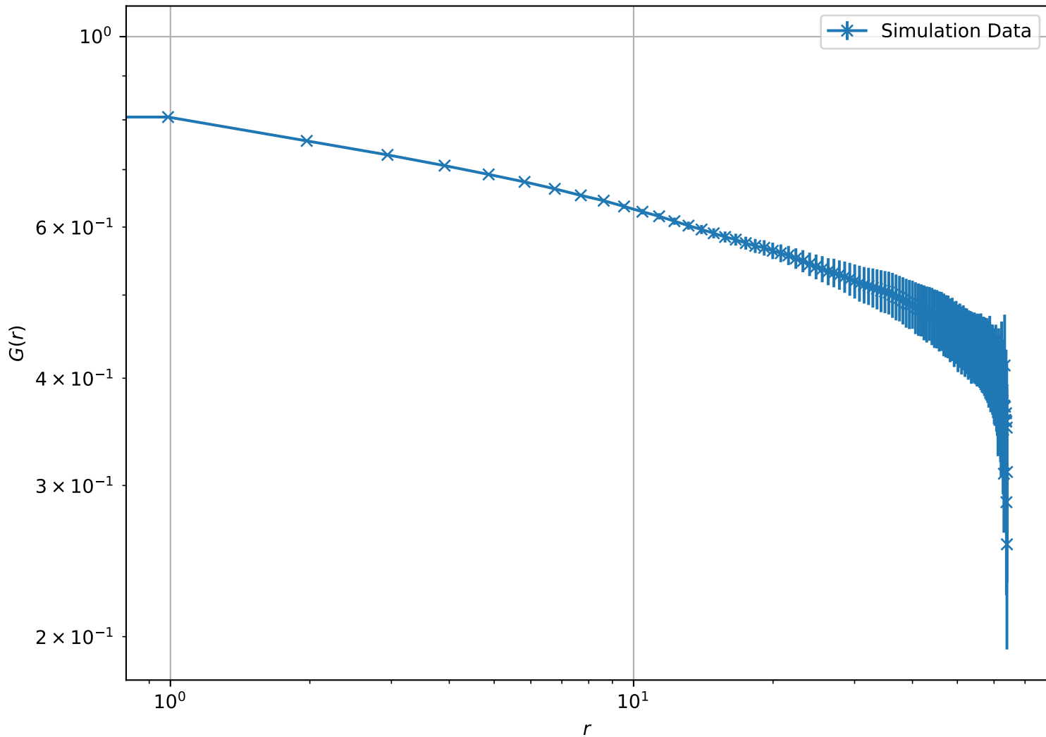
Correlation Function at T = 9.00e - 01 , L = 64 (Log-Log Scale)
