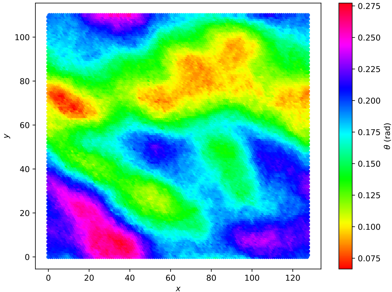
Hexagonal Lattice L=128 , T = 1.00e - 02
