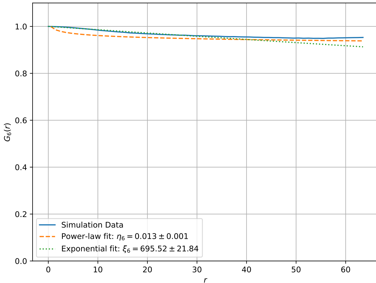
Correlation Function at T = 1.00e - 05, L = 128
