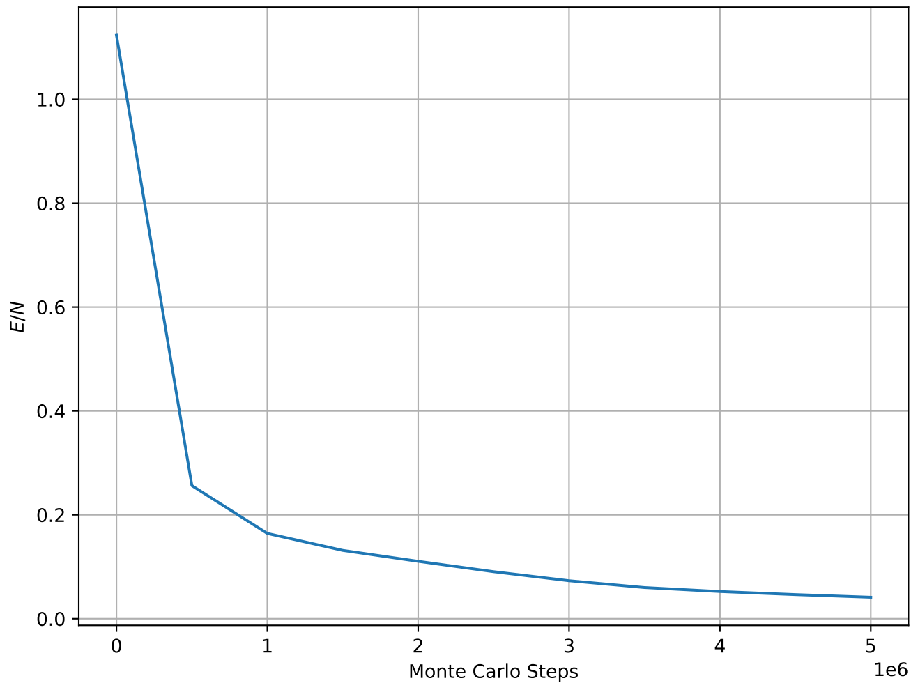
Energy per Spin at T = 1.00e - 05 , L = 128
