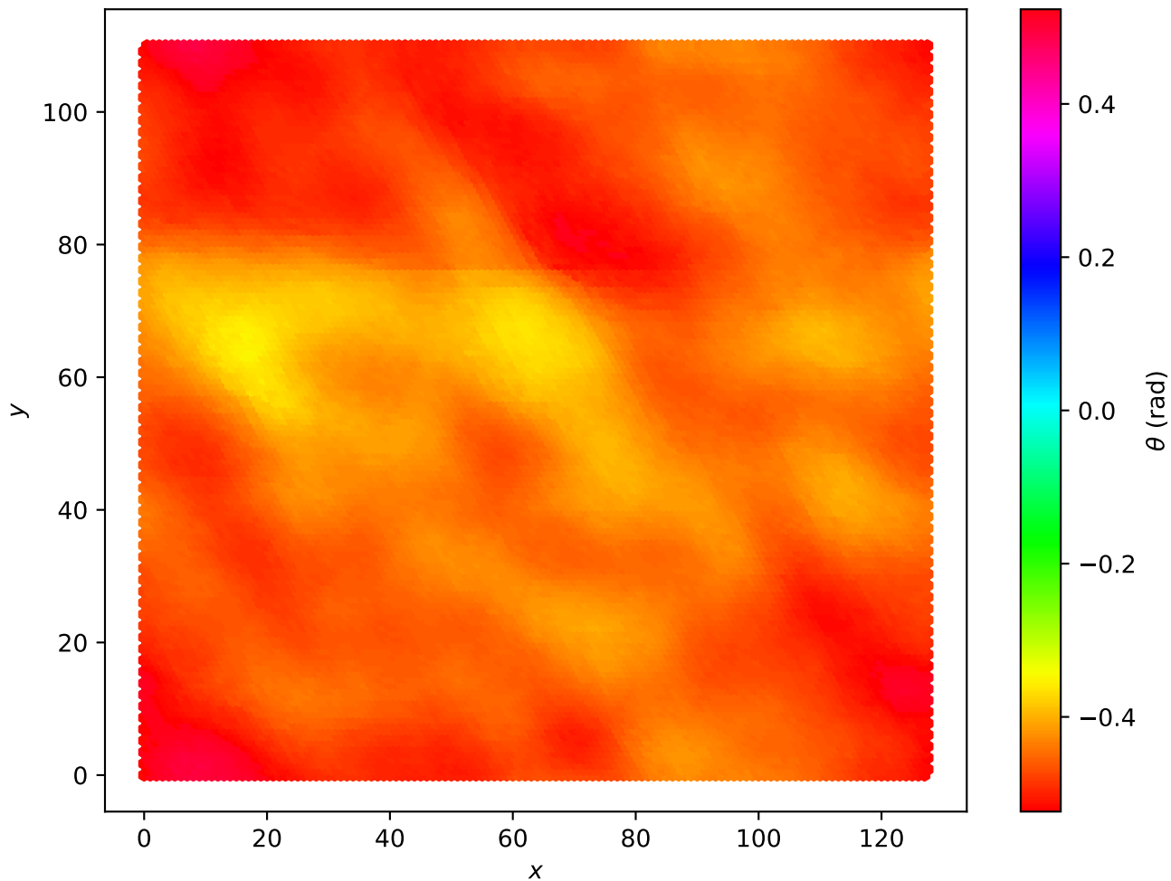
Hexagonal Lattice L=128 , T = 1.00e - 05
