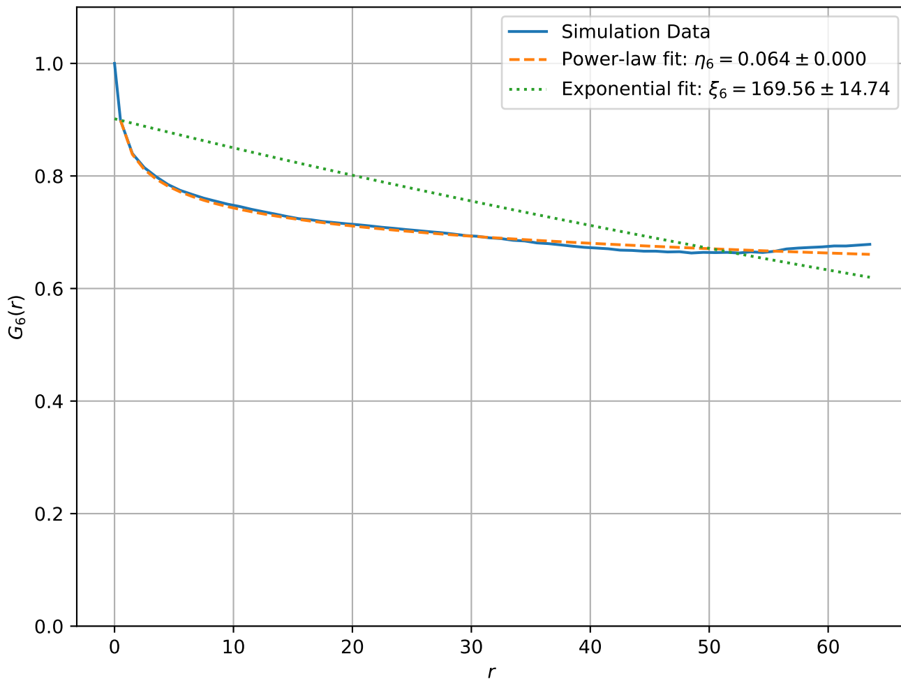
Correlation Function at T = 1.50e - 01, L = 128
