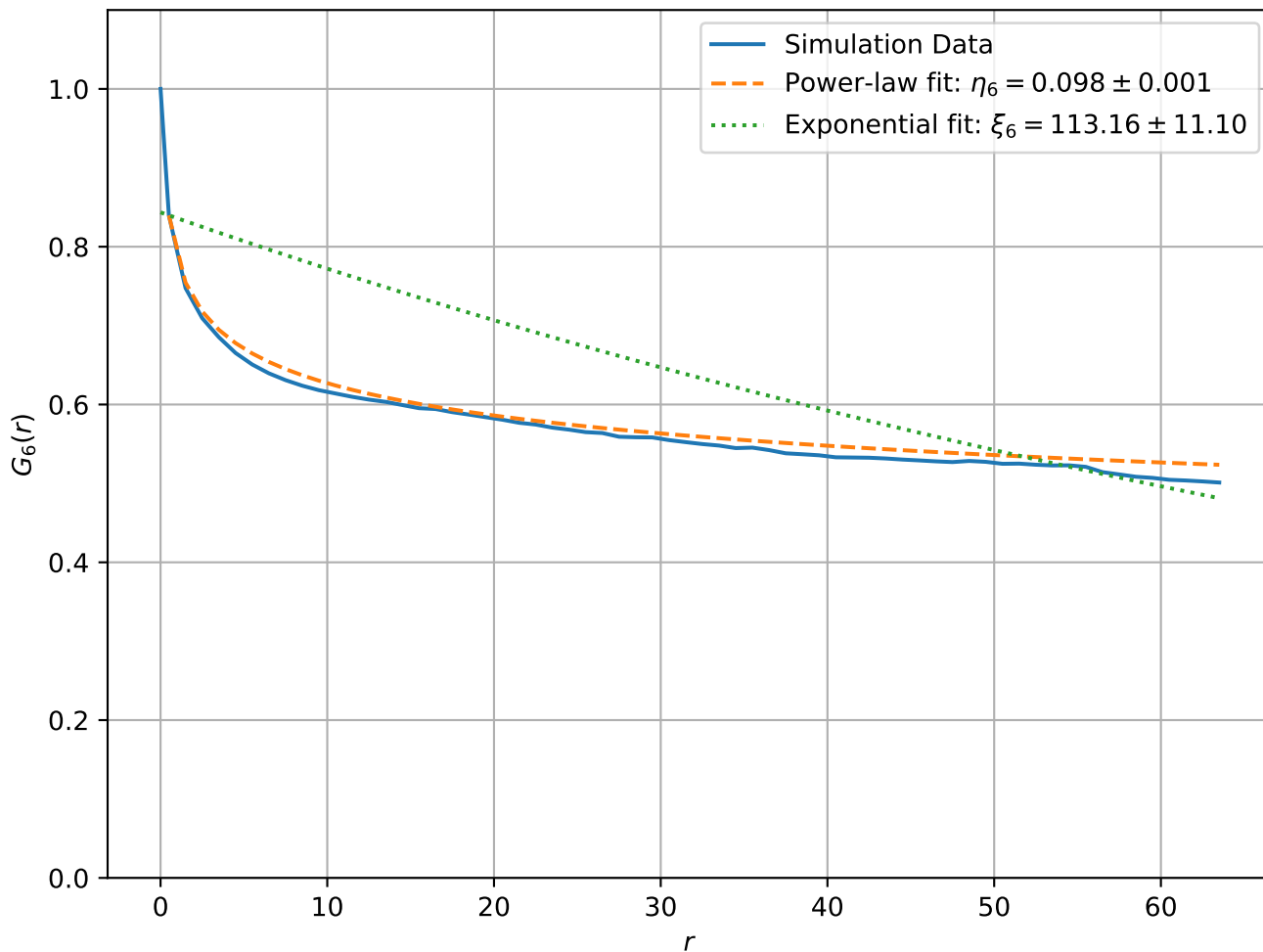
Correlation Function at T = 1.70e - 01 , L = 128
