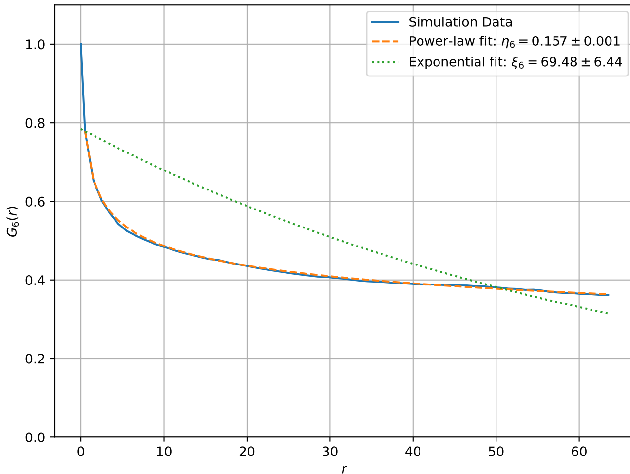
Correlation Function at T = 1.90e - 01, L = 128
