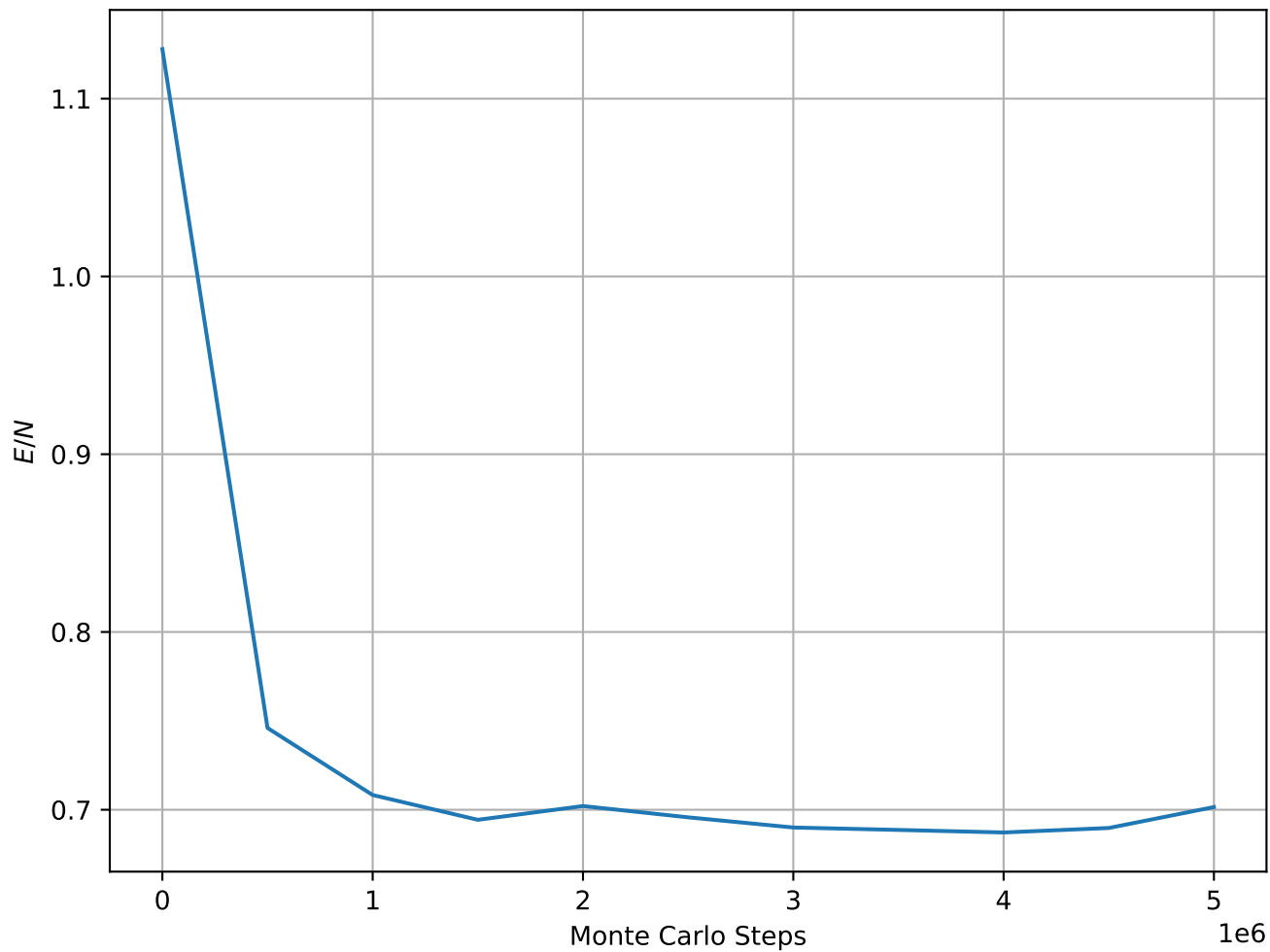
Energy per Spin at T = 2.00e - 01 , L = 128
