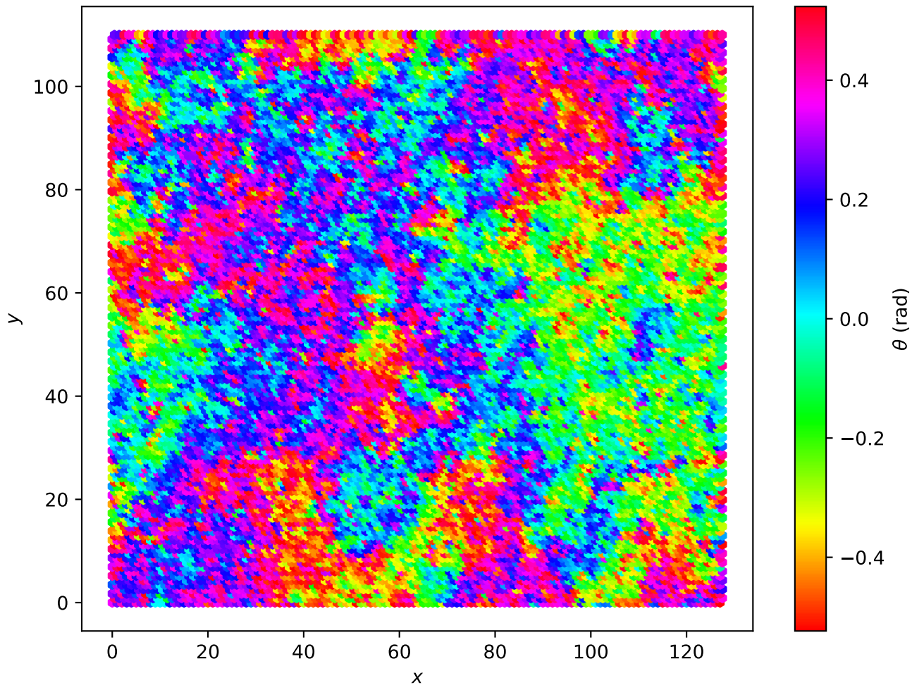
Hexagonal Lattice L=128 , T = 2.00e - 01
