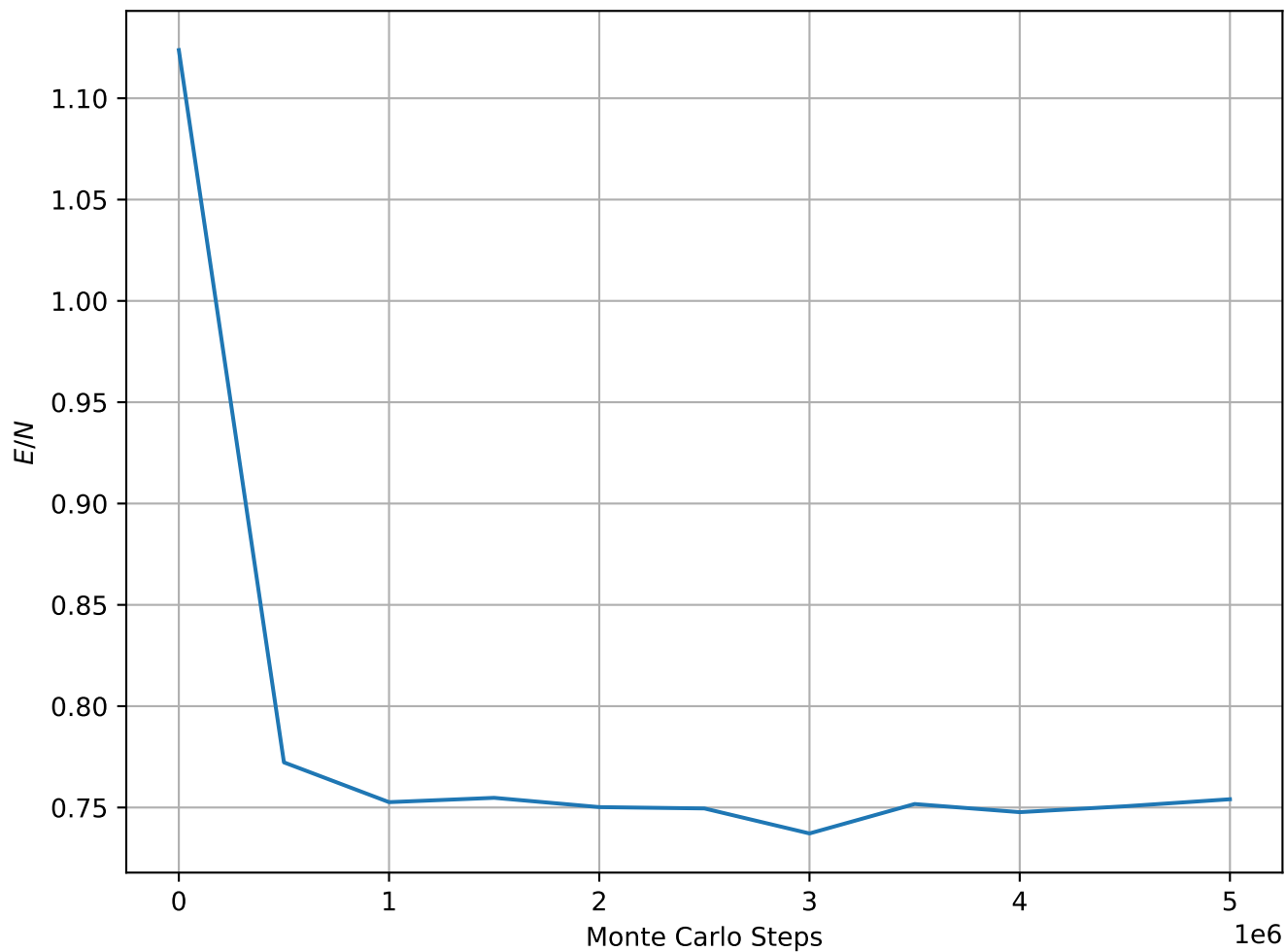
Energy per Spin at T = 2.10e - 01 , L = 128
