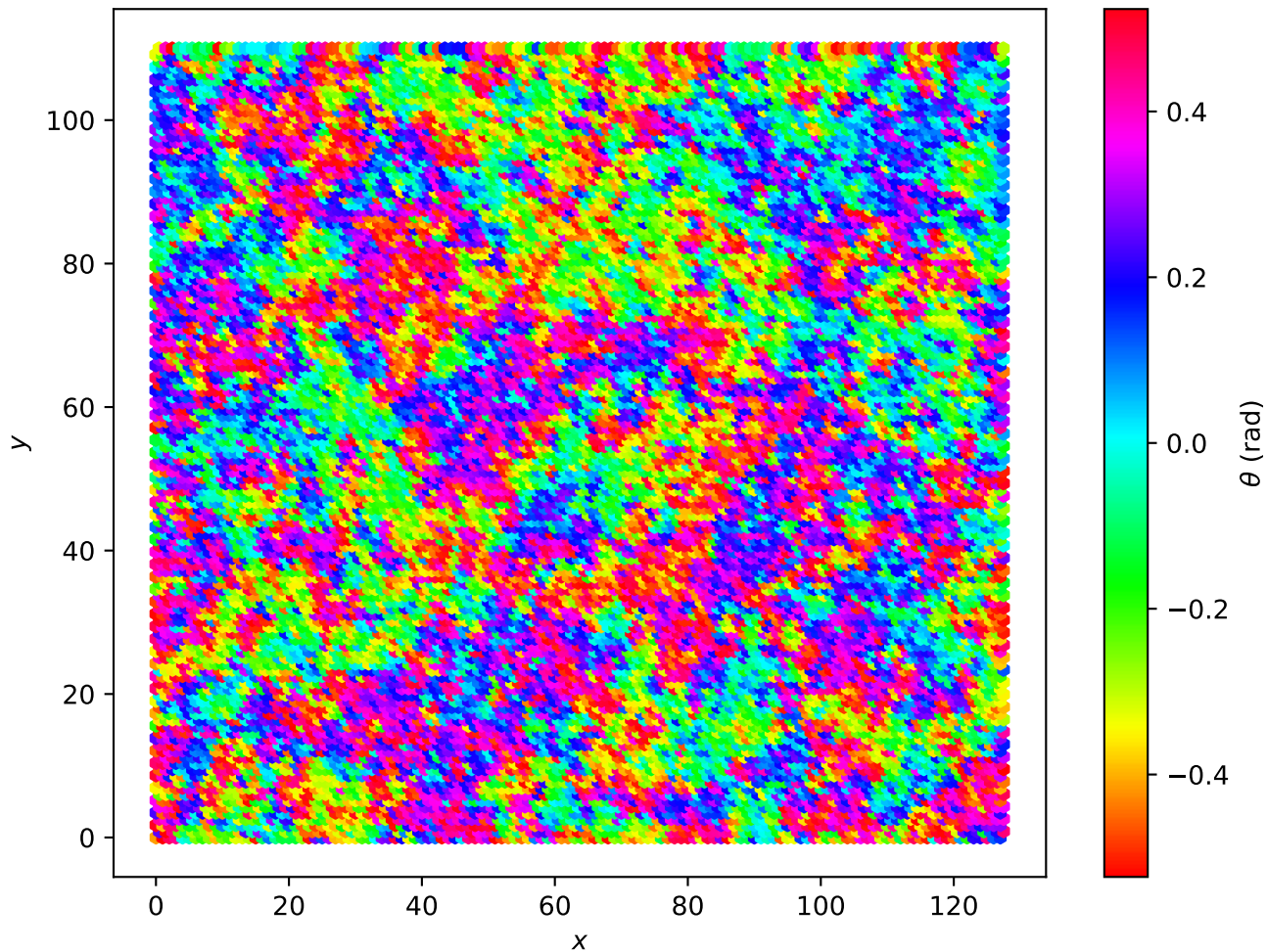
Hexagonal Lattice L=128 , T = 2.20e - 01
