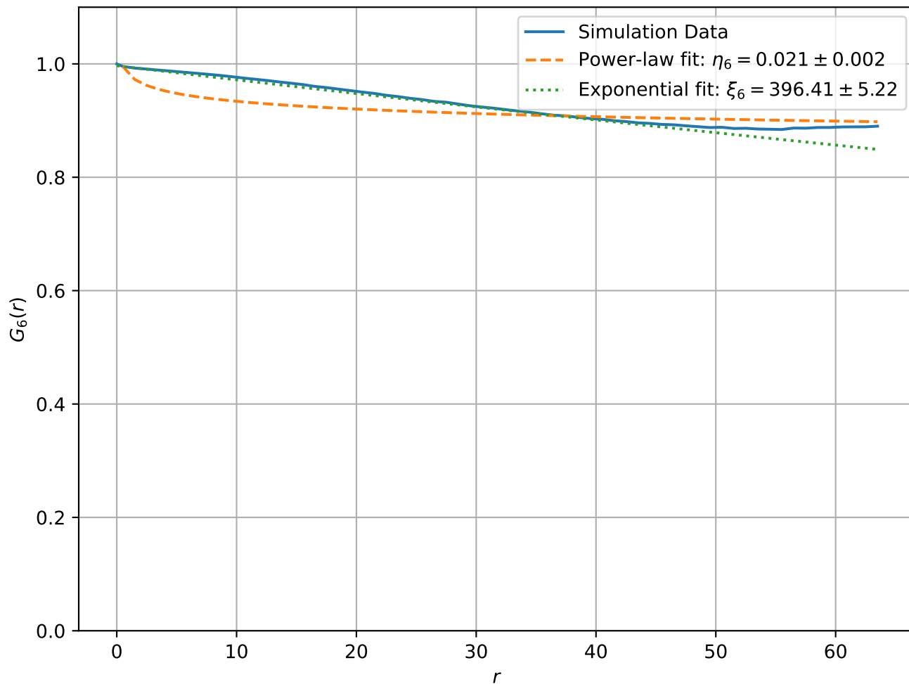
Correlation Function at T = 5.00e - 02 , L = 128
