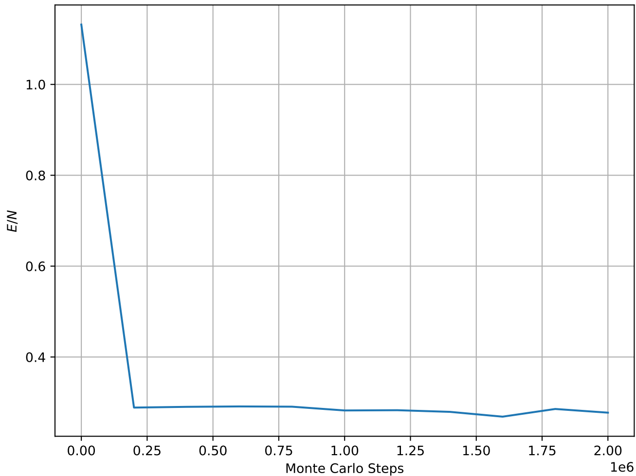
Energy per Spin at T = 1.00e - 01 , L = 32
