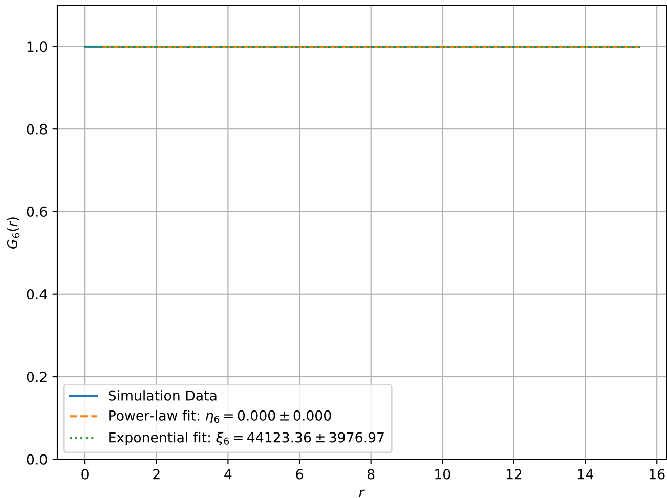
Correlation Function at T = 1.00e - 02 , L = 32
