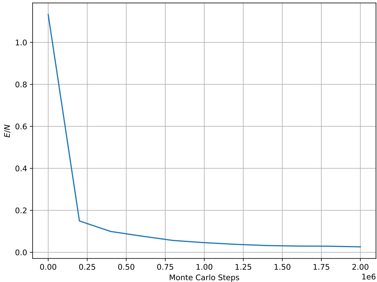
Energy per Spin at T = 1.00e - 02 , L = 32
