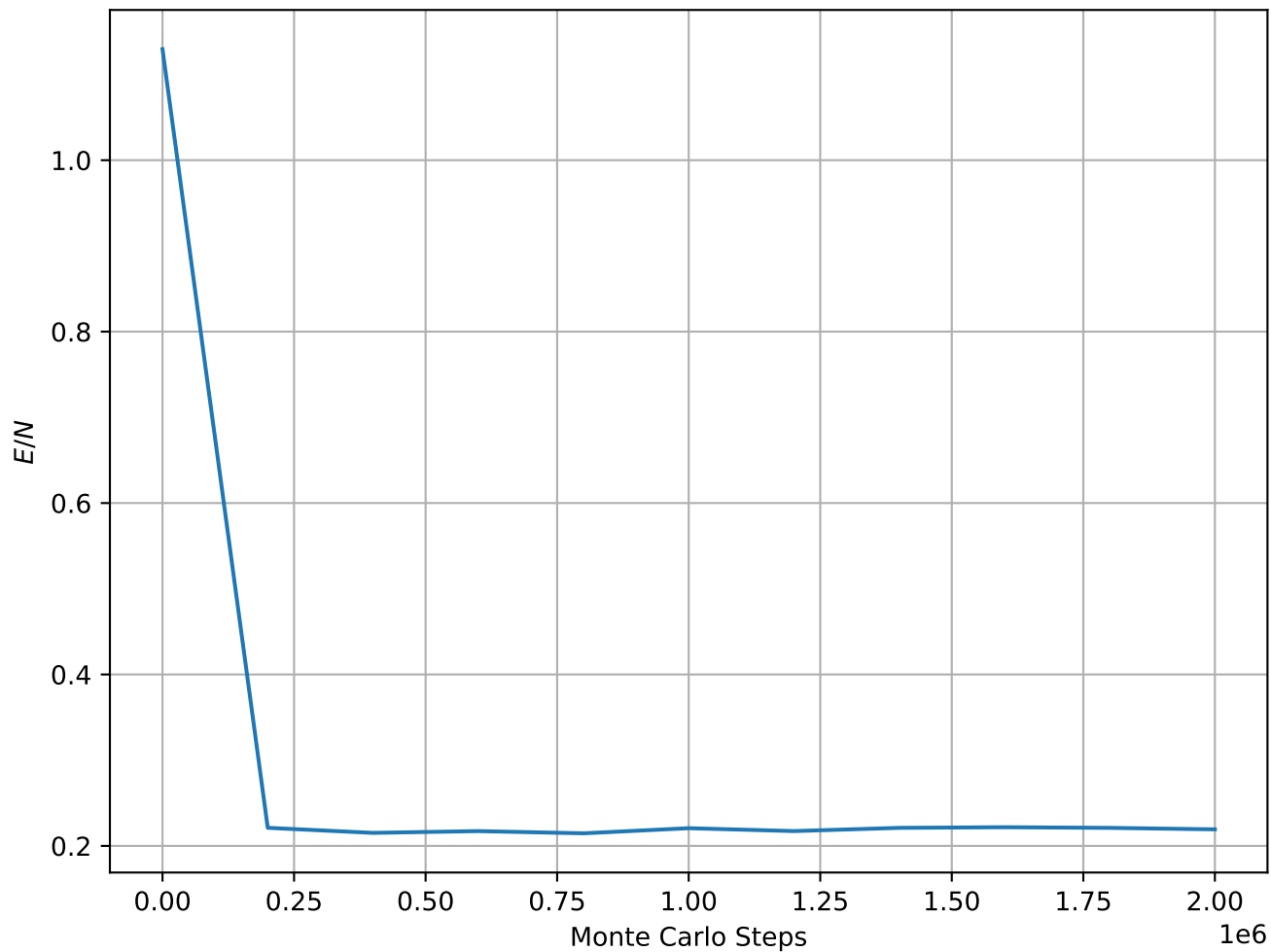
Energy per Spin at T = 1.00e - 05 , L = 32
