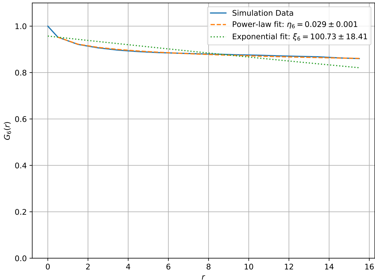
Correlation Function at T = 1.20e - 01 , L = 32
