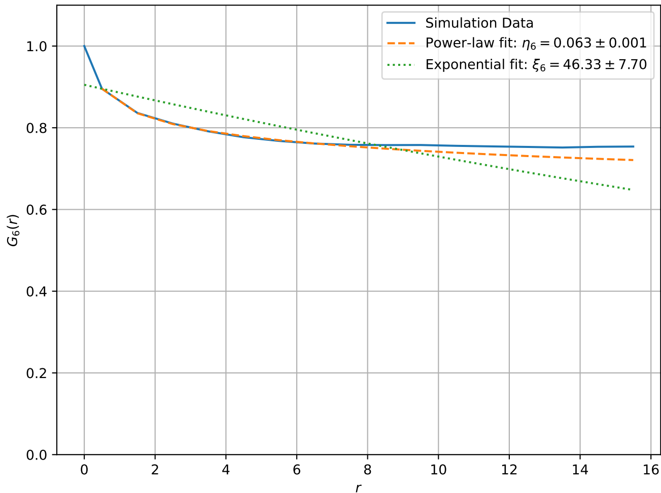
Correlation Function at T = 1.50e - 01 , L = 32
