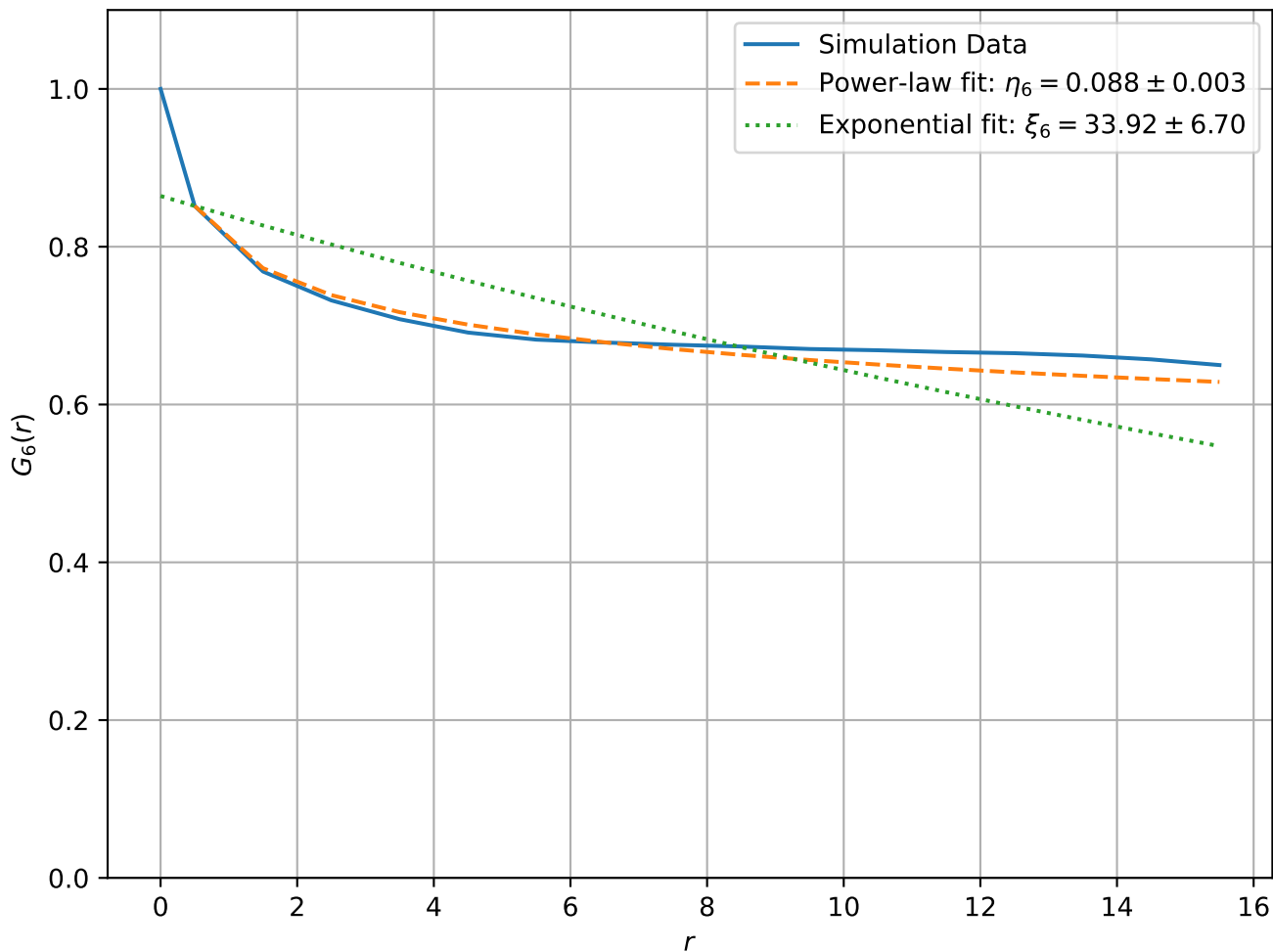
Correlation Function at T = 1.70e - 01 , L = 32
