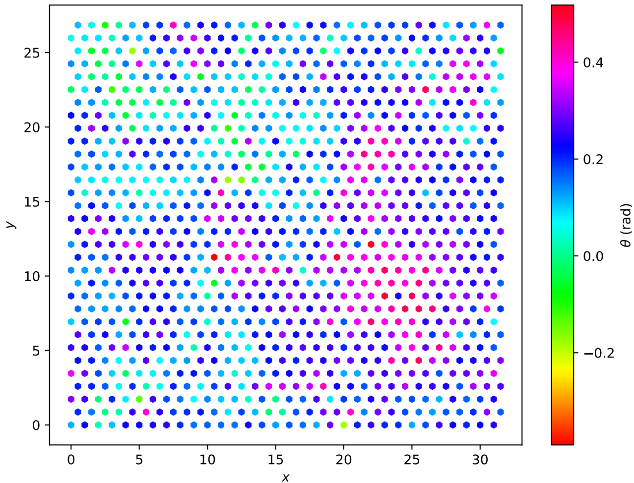
Hexagonal Lattice L=32 , T = 1.70e - 01
