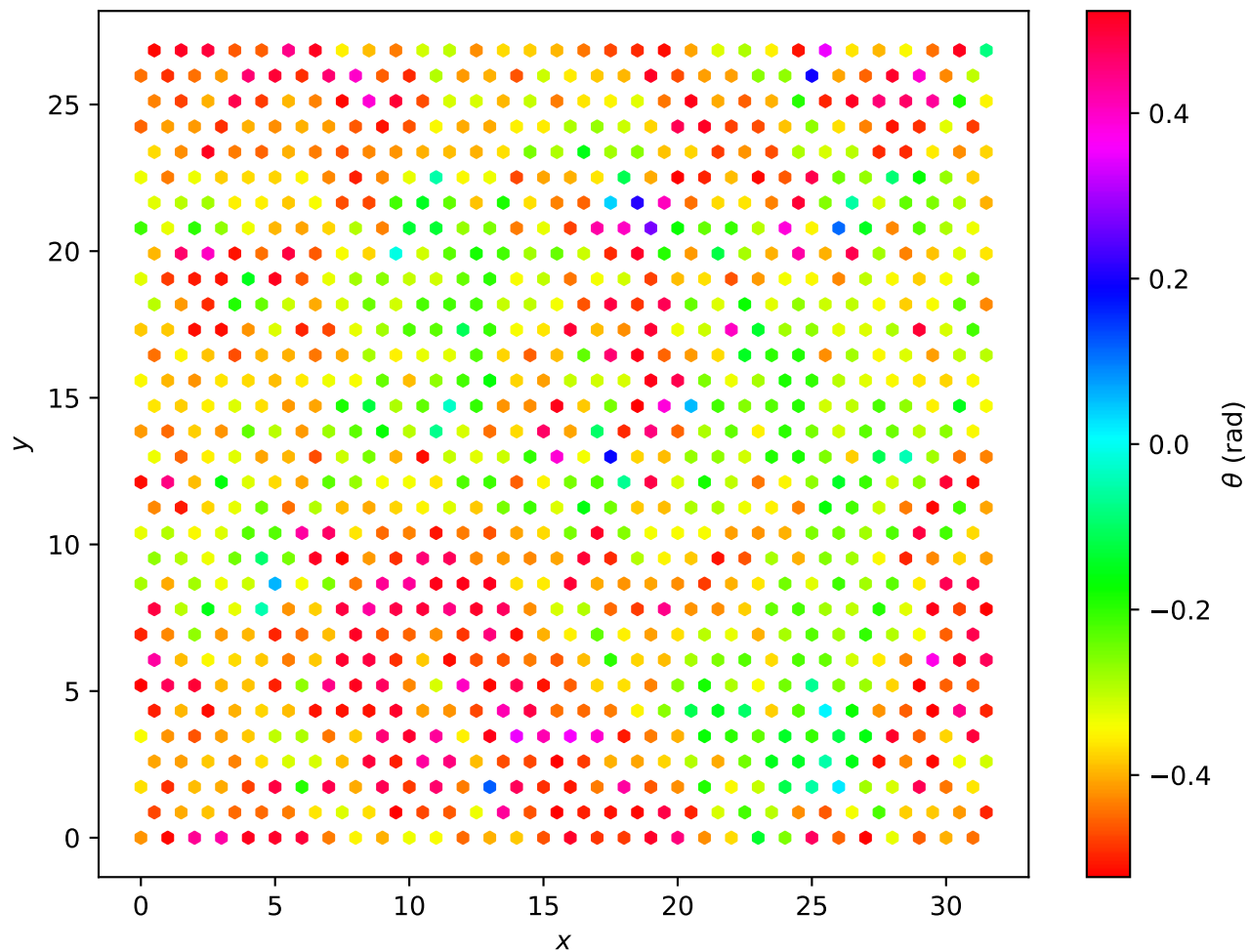
Hexagonal Lattice L=32 , T = 1.90e - 01
