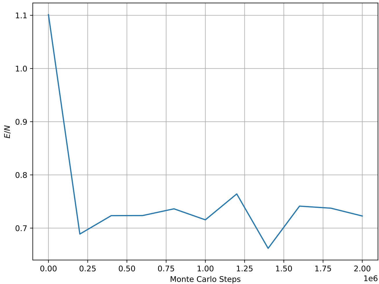
Energy per Spin at T = 2.10e - 01 , L = 32
