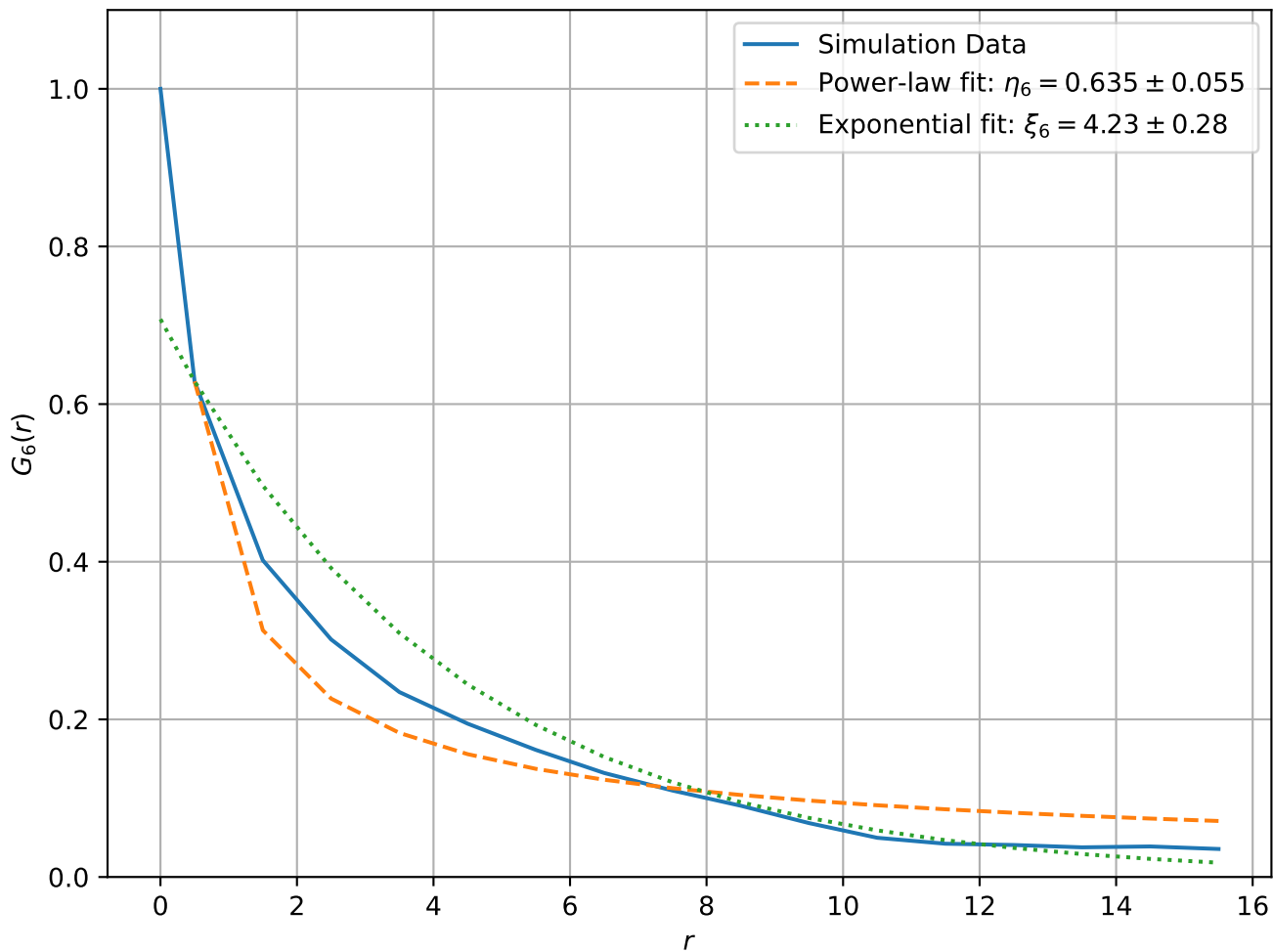
Correlation Function at T = 2.20e - 01 , L = 32
