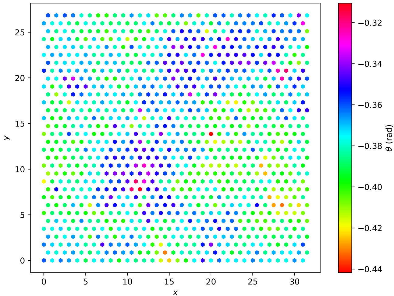
Hexagonal Lattice L=32 , T = 5.00e - 02
