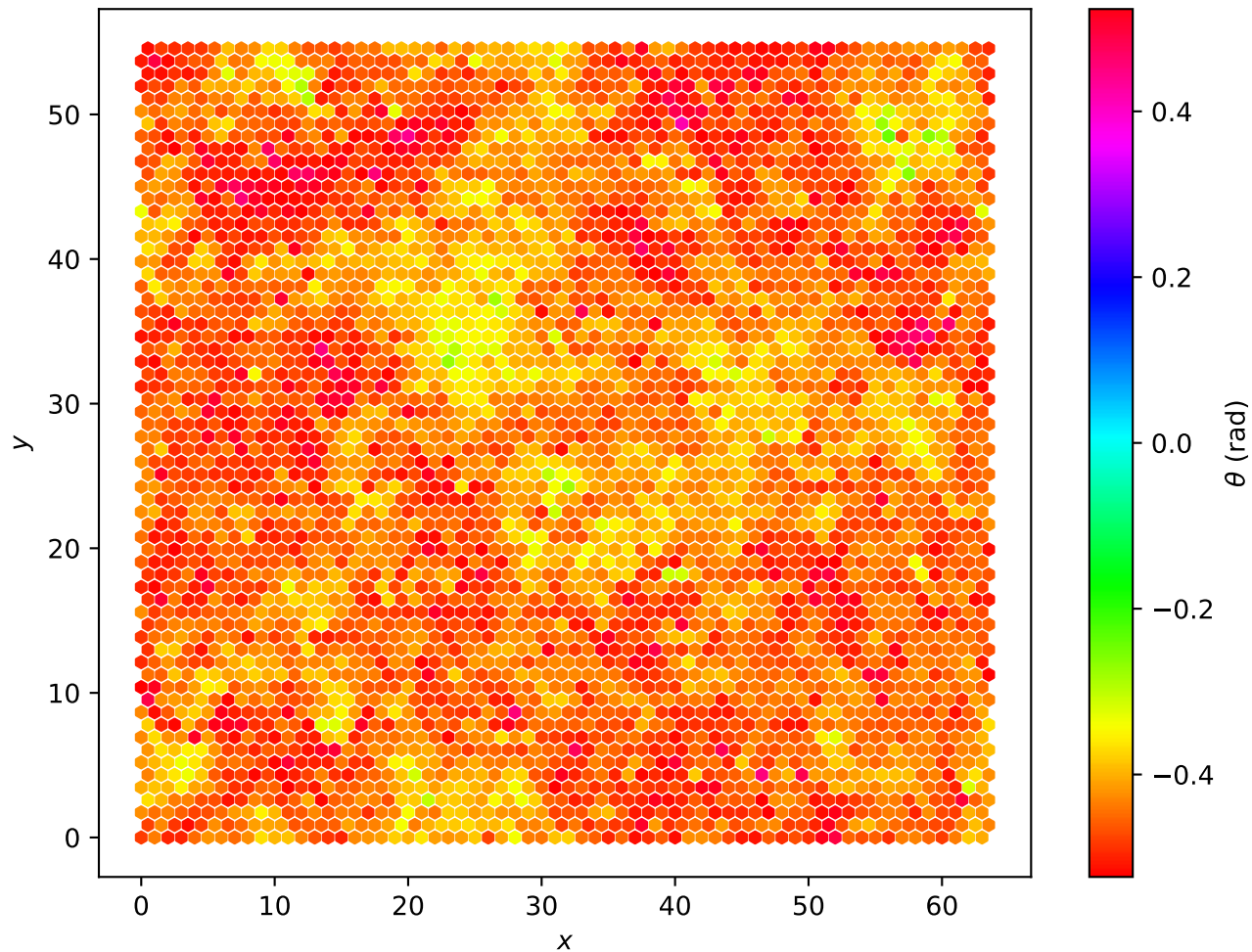
Hexagonal Lattice L=64 , T = 1.00e - 01
